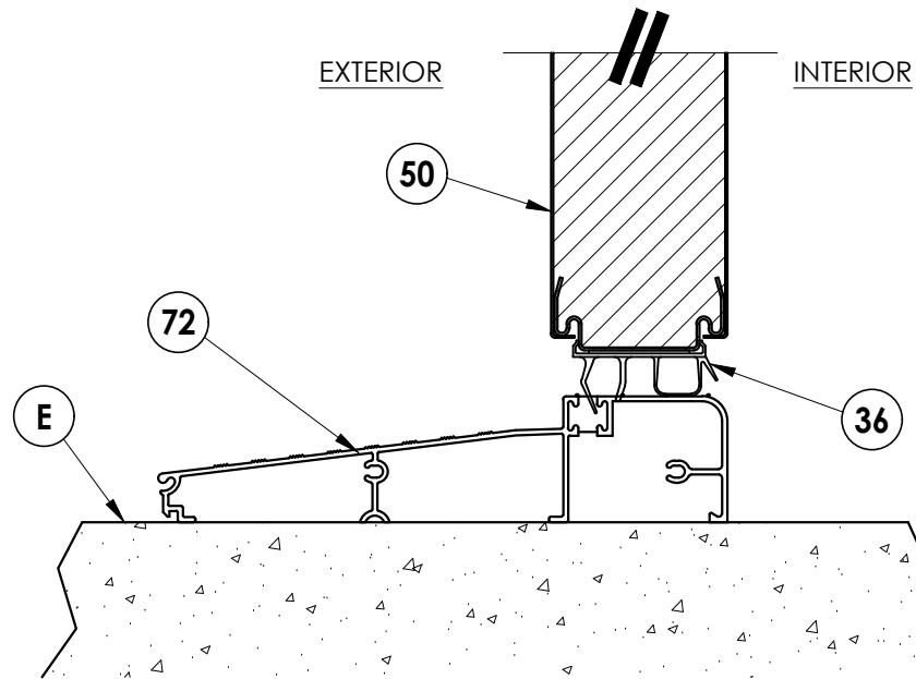
5 VERTICAL CROSS SECTION 5
