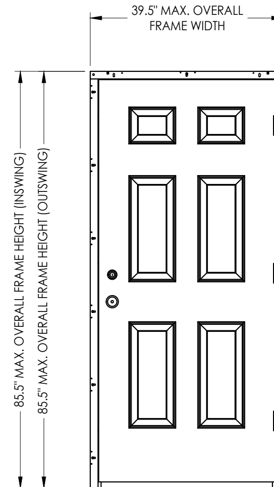
INSWING / OUTSWING
